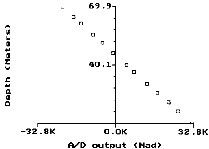
A/D Scaling
