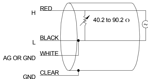
FIGURE 3-1. LI200X Schematic
